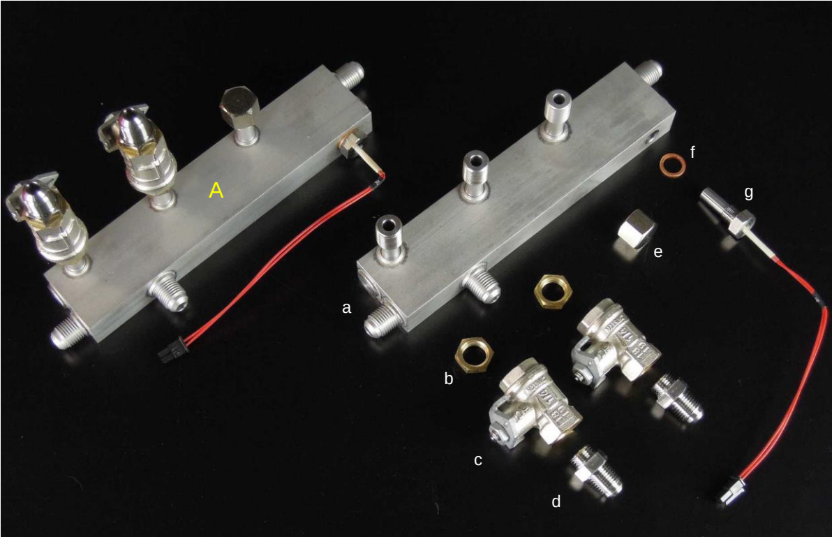
The photo shows at A the heat exchanger cooling block for a Duette. On the Triplette block, the female plug (e) is replaced with an extra ball-valve (b+c+d).
