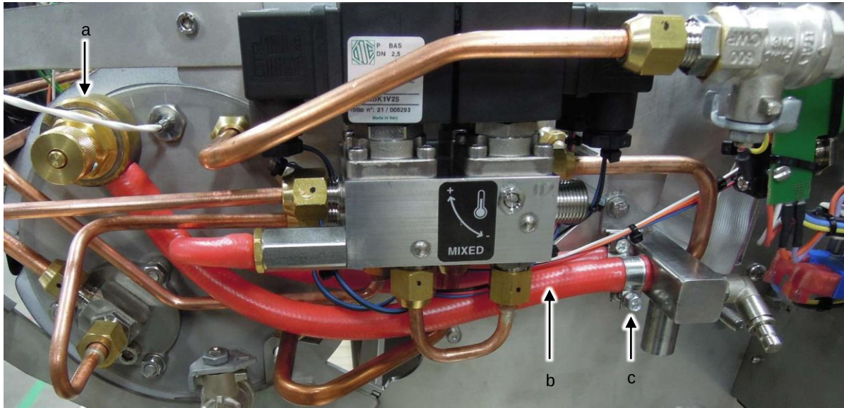
Showing the new version pressure safety valve.
