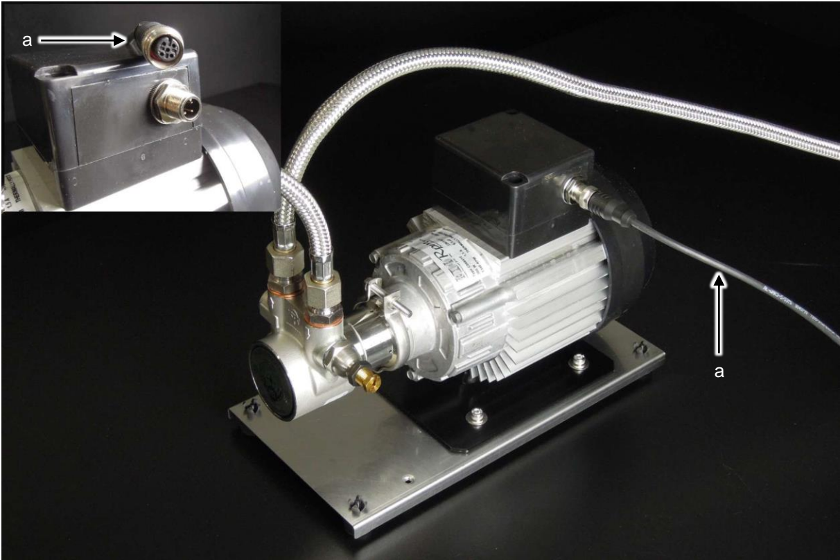
Pump with M12 plug-in pump-cable. This cable has a moulded plug.
